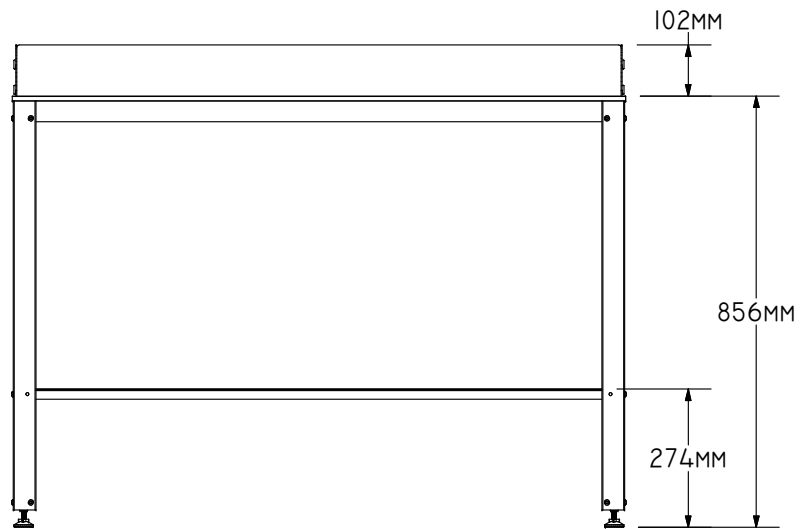
FRONT ELEVATION 1:15
